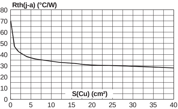
Fig. 10: Thermal resistance junction to ambient versus copper surface under tab (epoxy printed circuit board FR4, Cu=35μm) (D 2 PAK).
